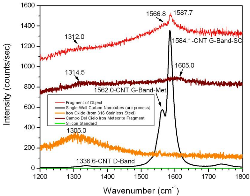
Figure 49-532 nm Raman Spectrum of Sample-as compared to iron oxide, a sample of iron meteorite, and single-walled carbon nanotubes-High Wave-Numbers
