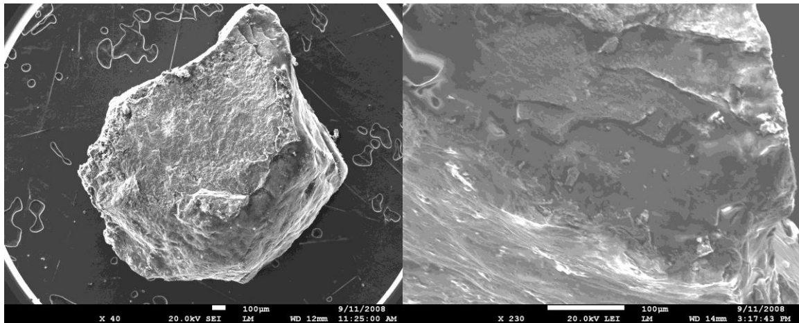
Figures 16 1 and 17-Low magnification Images of Sample (40X and 230X)- Showing whole sample and outer layer over darker bulk material
