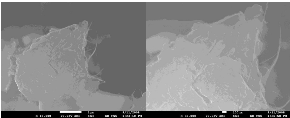
Figures 28 and 29-Higher Magnification Views of Light Material Inclusion in Dark Area of Sample-Showing Nanofibers (18,000X and 35,000X)
