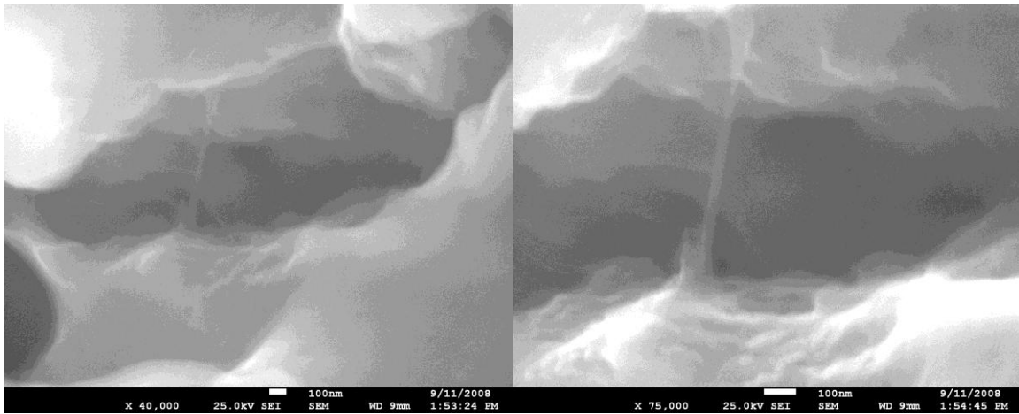
Figures 26 and 27-High Magnification Views of Cracks in Shiny Layer of Sample-Showing Nanofibers (40,000X and 75,000X)
