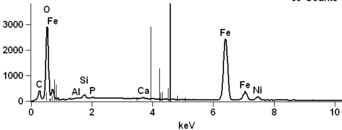
Figure 39- Small Area EDX Scan of Light and Dark Areas of the Sample
