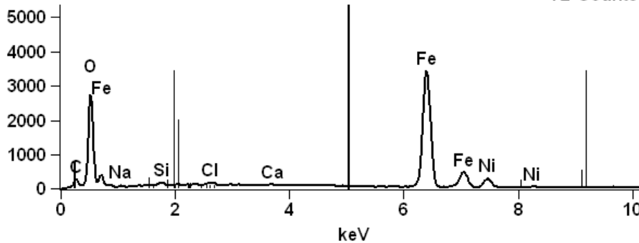
Figure 41- Small Area EDX Scan of Light Area of the Sample-Showing Bone-like Structure
