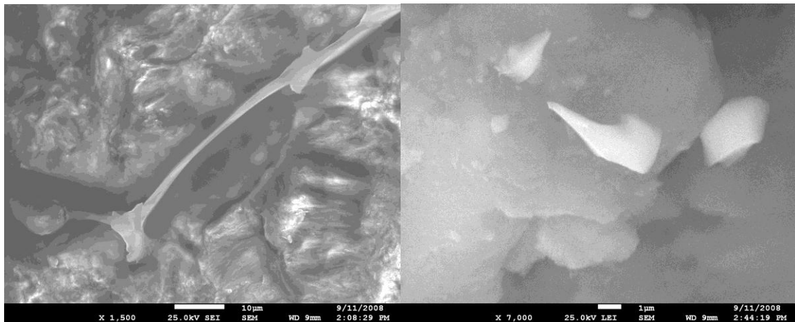
Figures 24 and 25-Views of Oddly Shaped Light Material Inclusions (1,500X and 7,000X)
