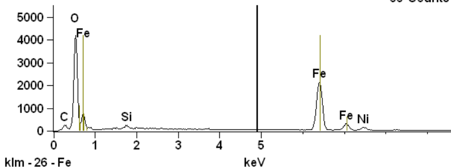
Figure 38-Small Area EDX Scan of Light
