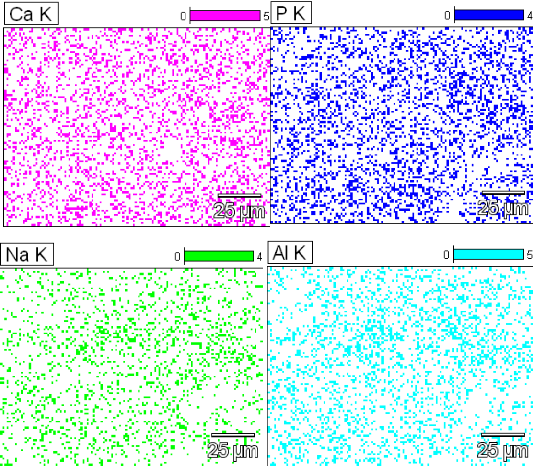
Figure 46 (continued)—EDX Elemental Mapping of Sample—Showing more Na and Al in Light Colored Inclusion
