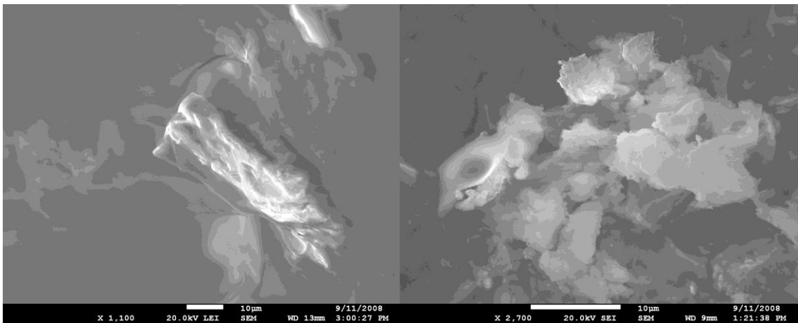
Figures 22 and 23-Inclusions of Light Material in Dark, Bulk, Area of Sample (1,100X and 2,700X)
