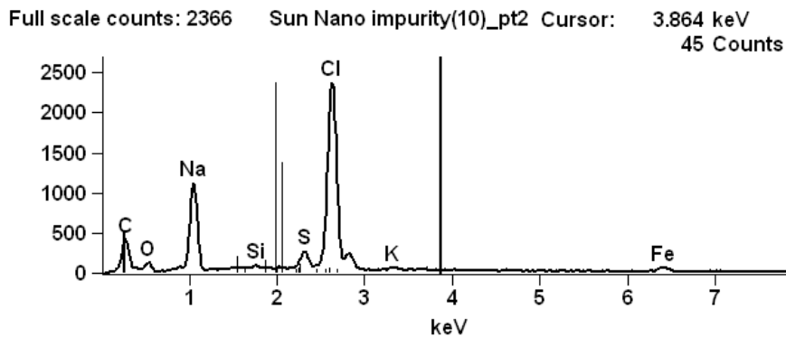
Figure 47- Small Area EDX Scan of Crystals and Adjacent Areas of Sample
