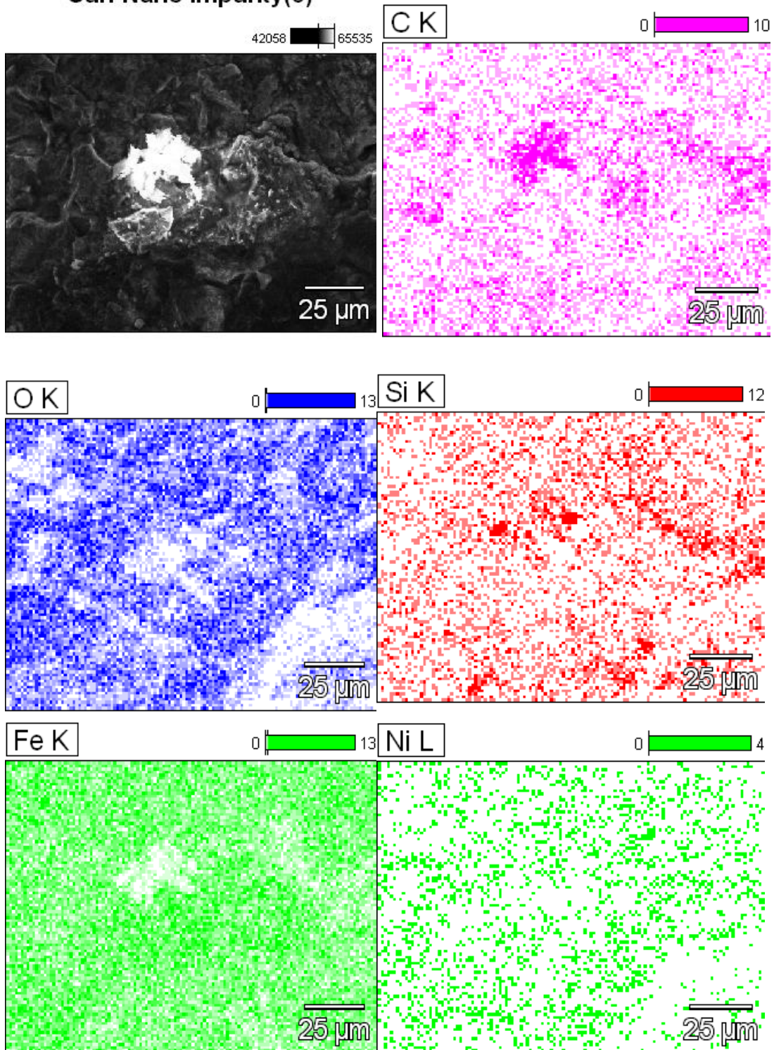
Figure 46—EDX Elemental Mapping of Sample—Showing less Fe and Ni, and more C, O, and Si in Light Colored Inclusion
