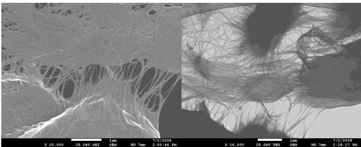
Figures 30 and 31-Single-Walled carbon Nanotubes (arc process)-Shown for Comparison
