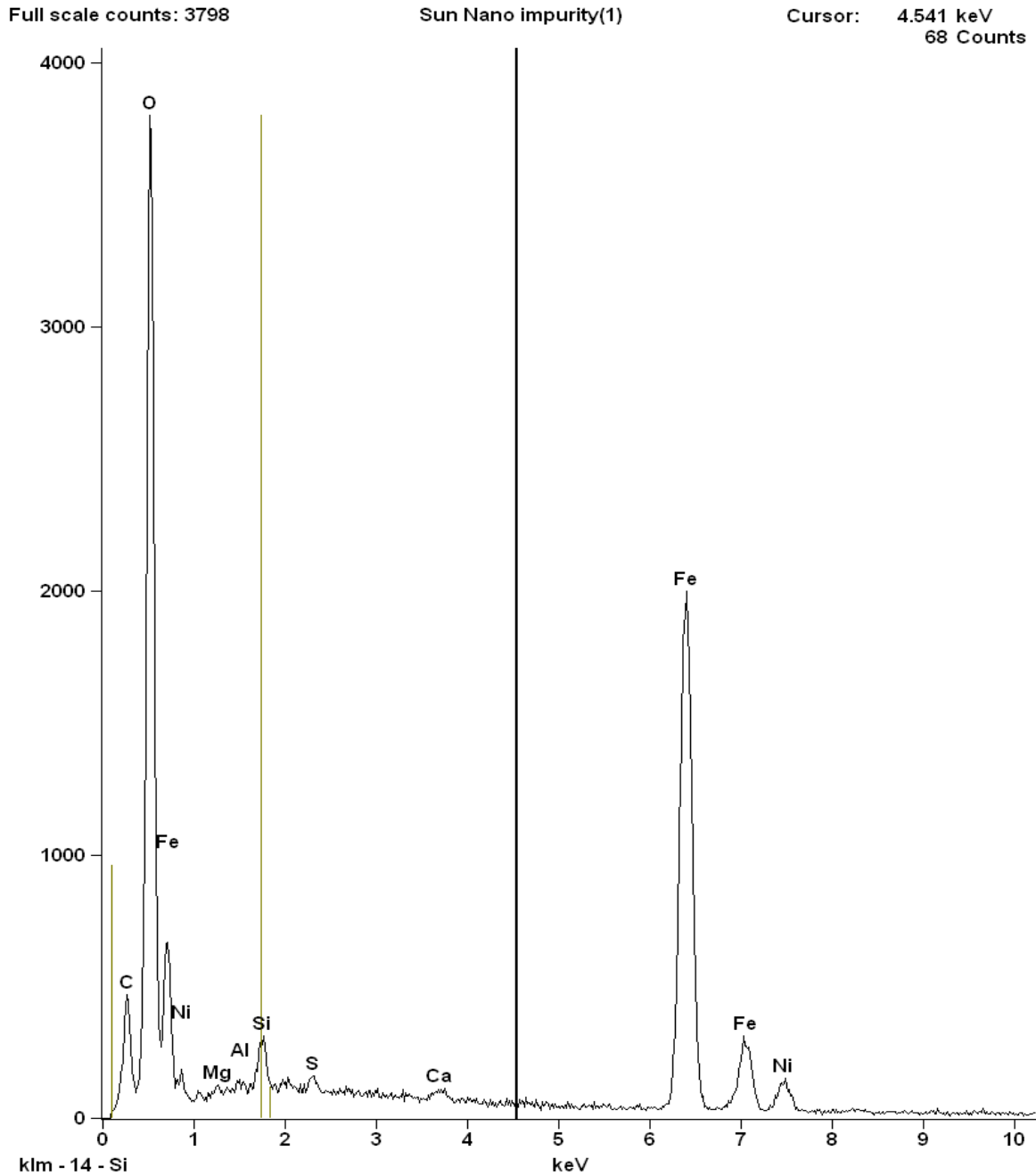
Figure 36-Large-Area EDX Scan of Object
