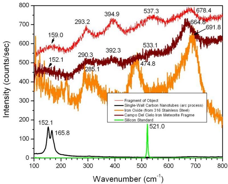
Figure 48-532 nm Raman Spectrum of Sample-as compared to iron oxide, a sample of iron meteorite, and single-walled carbon nanotubes-Low Wave-Numbers
