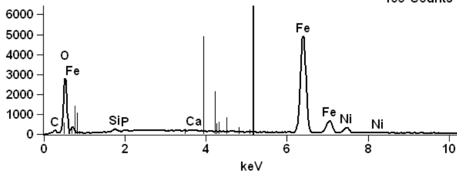
Figure 42- Small Area EDX Scan of Dark Area of the Sample-Showing Nanopit in Dark Material
