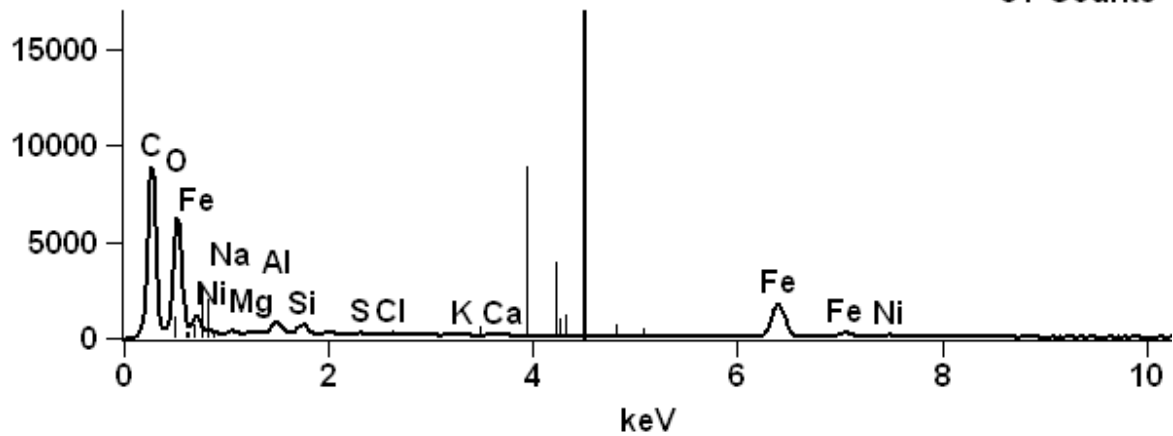
Figure 40- Small Area EDX Scan of Light Area of the Sample-Showing Nanotube Bundles
