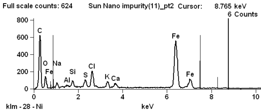
Figure 43- Small Area EDX Scan of Light Area of the Sample-Showing Horn-like Structure
