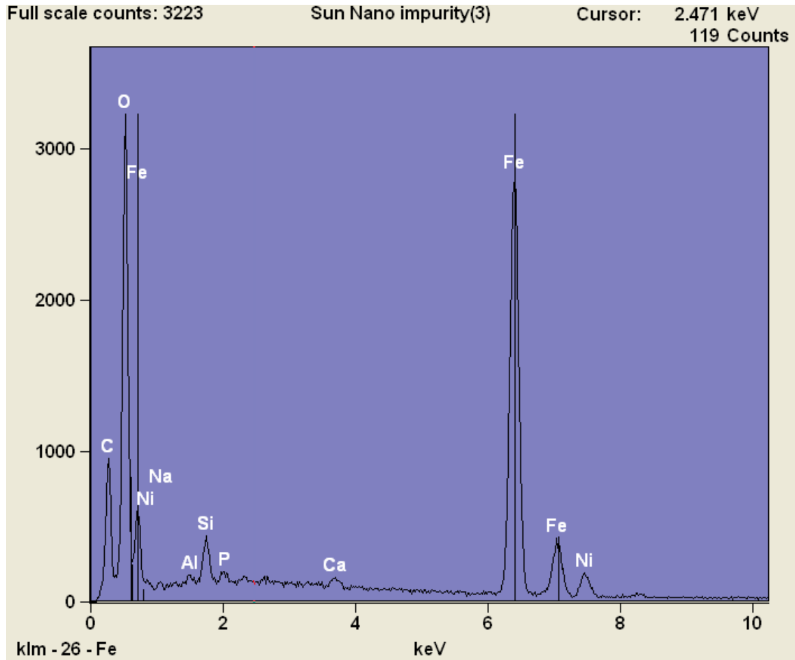
Figure 37-Second Large-Area EDX Scan of Object
